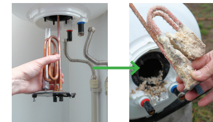
IMMERSION element in direct contact with the water (generally cheaper)
